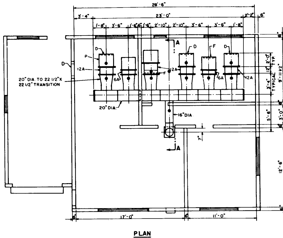
Fig. 2—Schematic diagram of ventilation system in concrete house.
